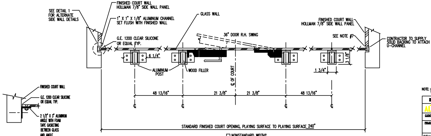
SECTION "A"
