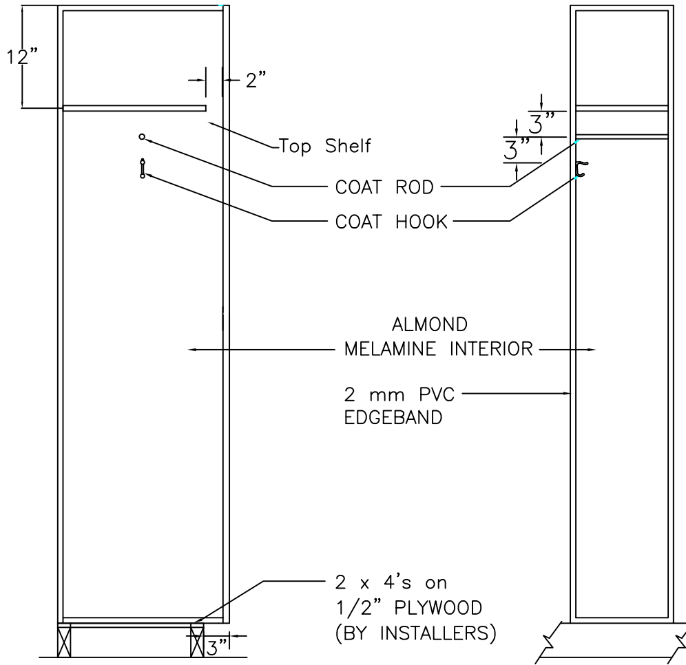
SECTION VIEW
