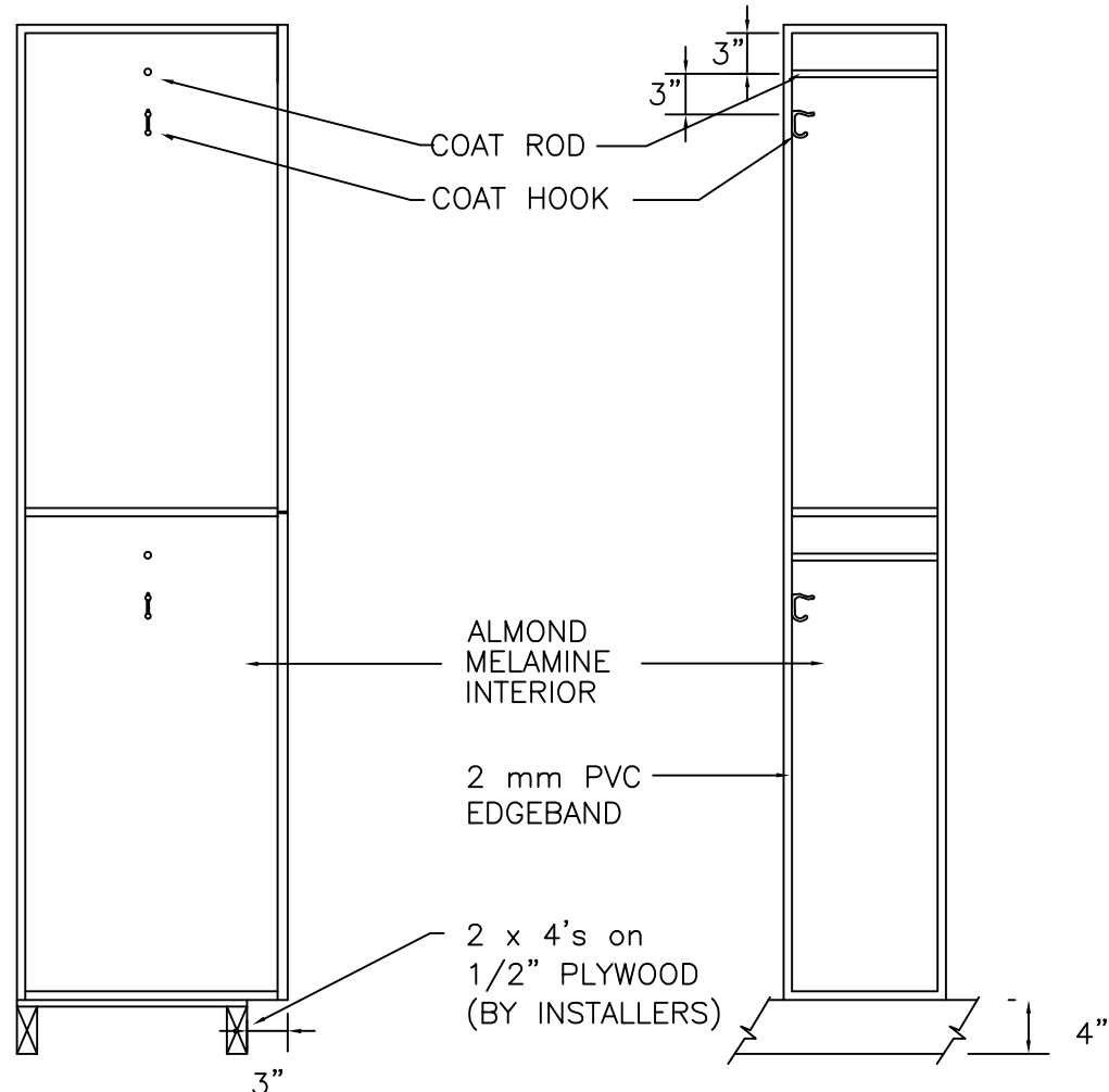
SECTION VIEW
