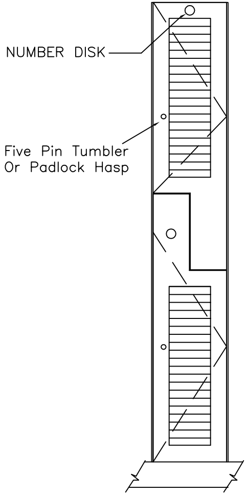
FRONT ELEVATION
