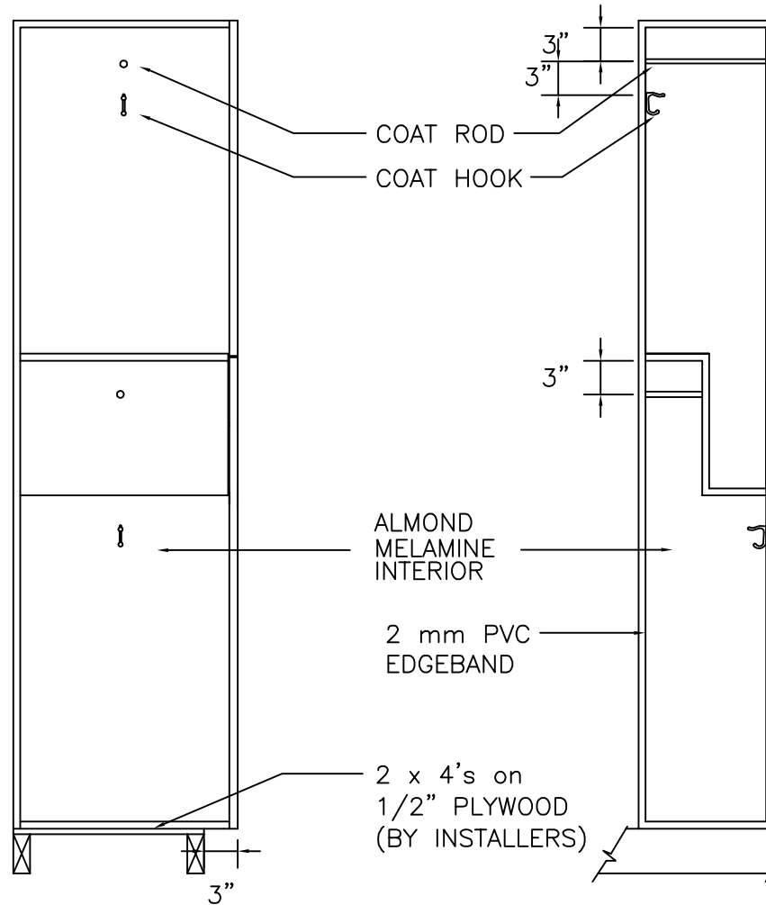
SECTION VIEW
