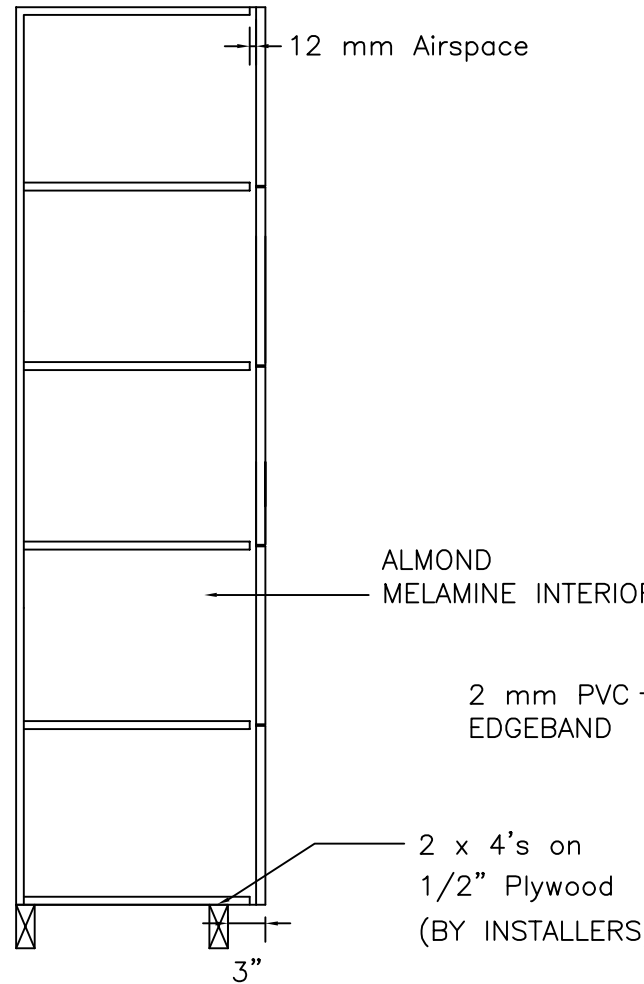
SECTION VIEW
