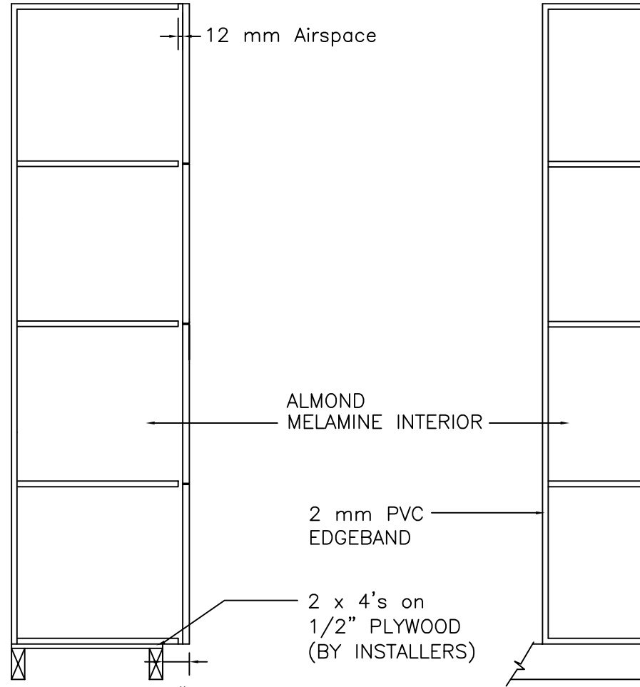
SECTION VIEW
