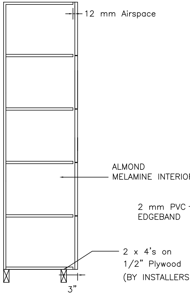
SECTION VIEW
