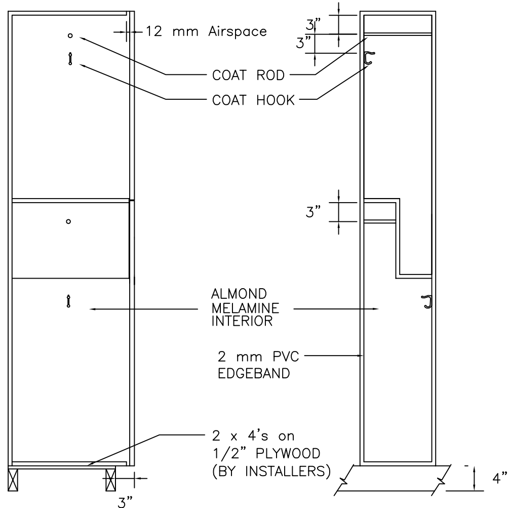
SECTION VIEW
