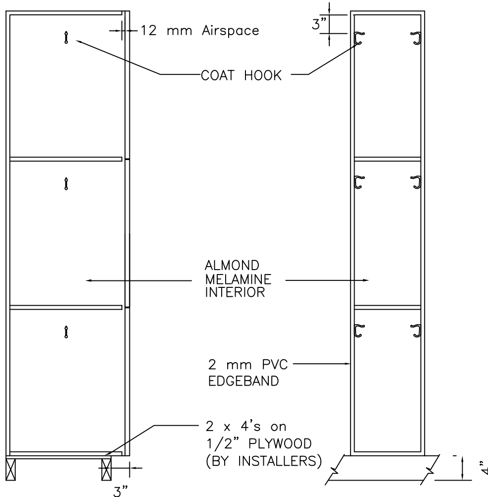
SECTION VIEW
